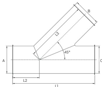
Branch pieces AISI 304/316 45°
