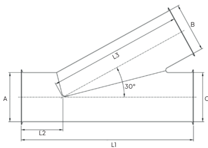
Branch pieces AISI 304/316 30°
