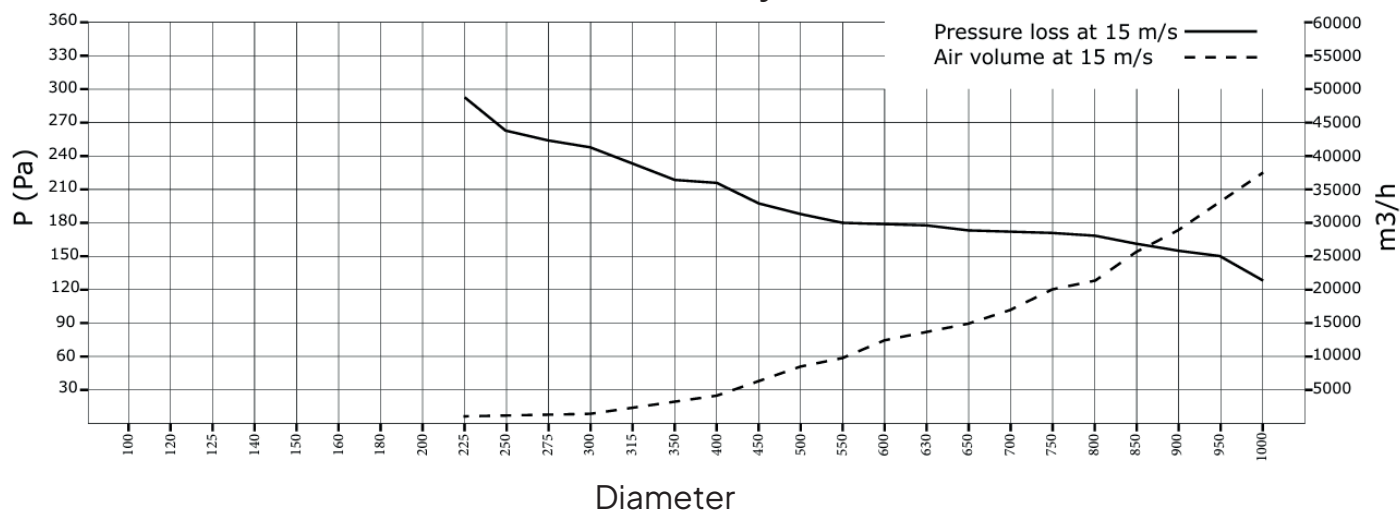
GASI-B L=1000 mm trykkfallstabell
